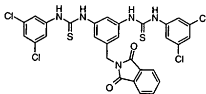
Compound # 27
